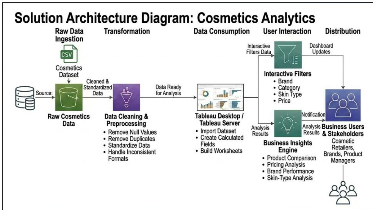
Figure 1: Architecture of Cosmetics Insights project
